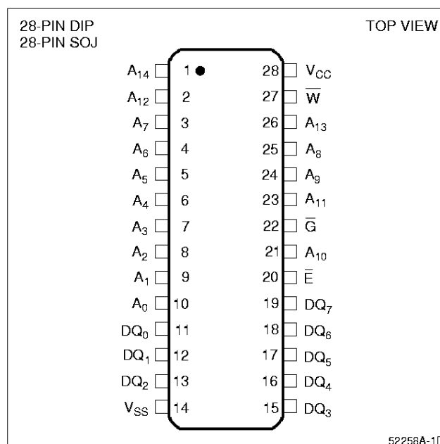
Figure 1. Pin Connections for DIP and SOJ Packages
