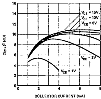
Figure 7. Typical |S_{21}|^2 vs. Bias at 2 GHz, for the HXTR-6103.
