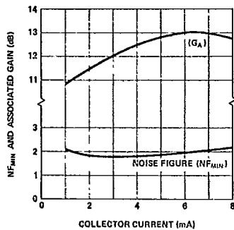
Figure 10. Typical N_{F_{MIN}} and Associated Gain vs. Collector Current at 2 GHz for V_{CE} = 10 V (Tuned for N_{F_{MIN}} ), for the HXTR-6103.
