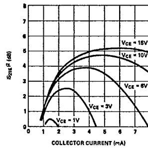
Figure 6. Typical |S_{21}|^2 vs. Bias at 4 GHz, for the HXTR-6101 and HXTR-6102.
