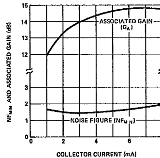
Figure 11. Typical Noise Figure and Associated Gain vs. I_C at 1.5 GHz for V_{CE} = 10 V (Tuned for N_{F_{MIN}} ) for the HXTR-6104.
