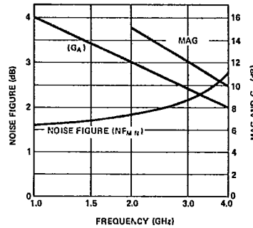
Figure 3. Typical MAG, Noise Figure (NF MIN ) and Associated Gain vs. Frequency (V CR = 10 V, I C = 3 mA), for the HXTR-6103.
