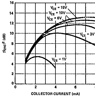
Figure 8. Typical |S_{21}|^2 vs. Bias at 1.5 GHz, for the HXTR-6104.
