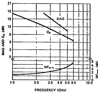
Figure 1. Typical MAG, Noise Figure (NF MIN ), and Associated Gain vs. Frequency (V CR = 10 V, I C = 4 mA), for the HXTR-6001.
