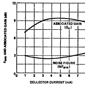
Figure 9. N_{F_{MIN}} and G , vs. Collector Current at 4 GHz for V_{CE} = 10 V, for the HXTR-6101 and HXTR-6102.
