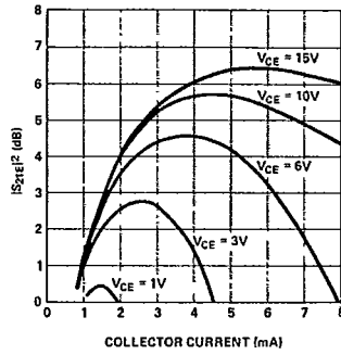
Figure 5. Typical |S_{21}|^2 vs. Bias at 4 GHz, for the HXTR-6001.
