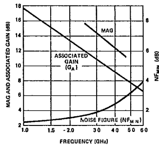
Figure 2. Typical MAG, Noise Figure (NF MIN ) and Associated Gain vs. Frequency (V CR = 10 V, I C = 4 mA), for the HXTR-6101 and HXTR-6102.
