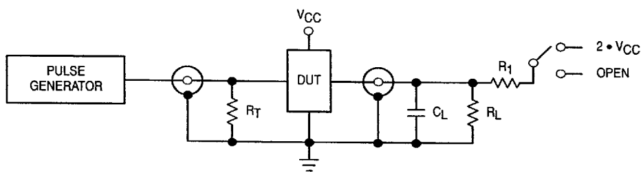
Figure 1. AC Waveforms
