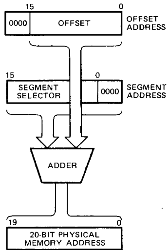
Fig. 8 – MBL 8086 REAL ADDRESS MODE ADDRESS CALCULATION
