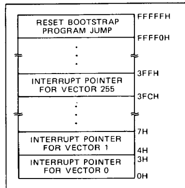
Fig. 9 – MBL 8086 REAL ADDRESS MODE INITIALLY RESERVED MEMORY LOCATIONS
