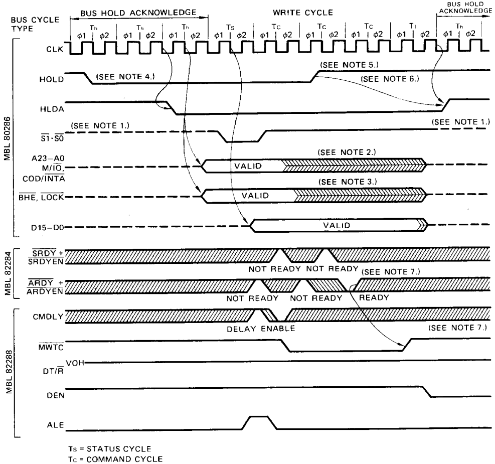
Fig. 29 – MULTIBUS WRITE TERMINATED BY ASYNCHRONOUS READ WITH BUS HOLD
