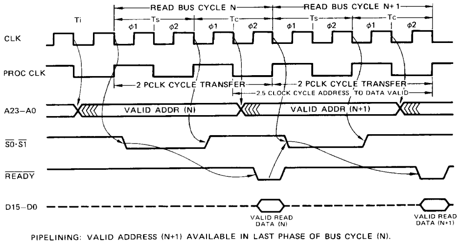
Fig. 23 – BASIC BUS CYCLE
