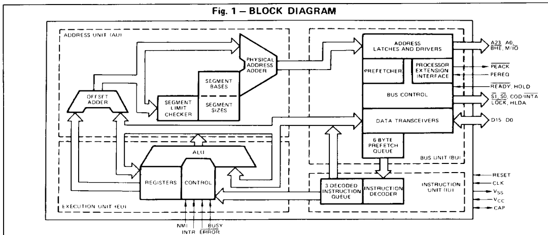
Fig. 1 – BLOCK DIAGRAM
