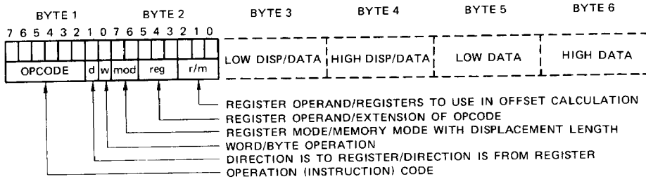
A. SHORT OPCODE FORMAT EXAMPLE
