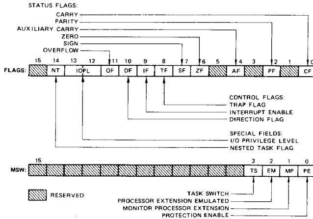
Fig. 3a – STATUS AND CONTROL REGISTER BIT FUNCTIONS
