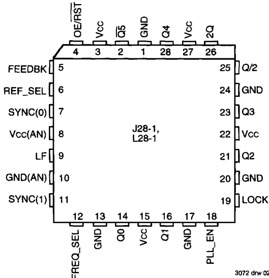
PLCC/LCC TOP VIEW
