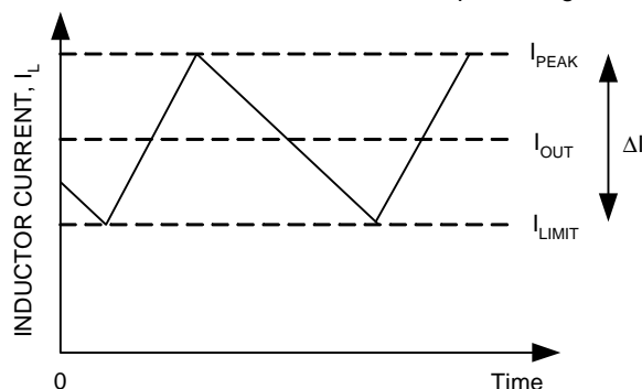
Figure 2. Current-Limit Algorithm
