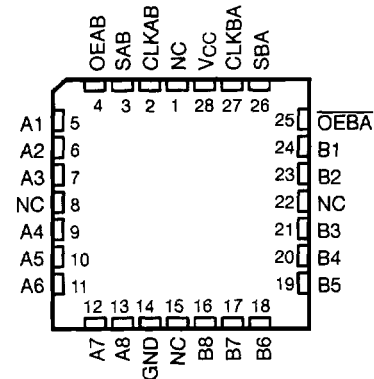
SN54BCT652 . . . FK PACKAGE (TOP VIEW)
