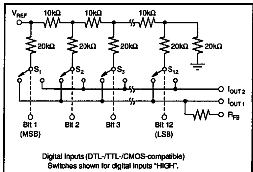
FIGURE 1. Simplified DAC Circuit.
