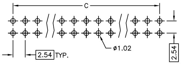
RECOMMEND P.C.B. LAYOUT BOTTOM VIEW
