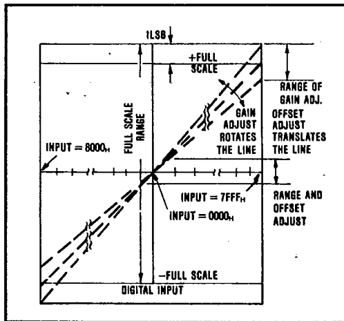
FIGURE 5. Relationship of Zero and Gain Adjustments for Bipolar D/A Converters, DAC705/706/707 and DAC708/709.
