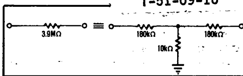
FIGURE 3. Equivalent Resistances.
