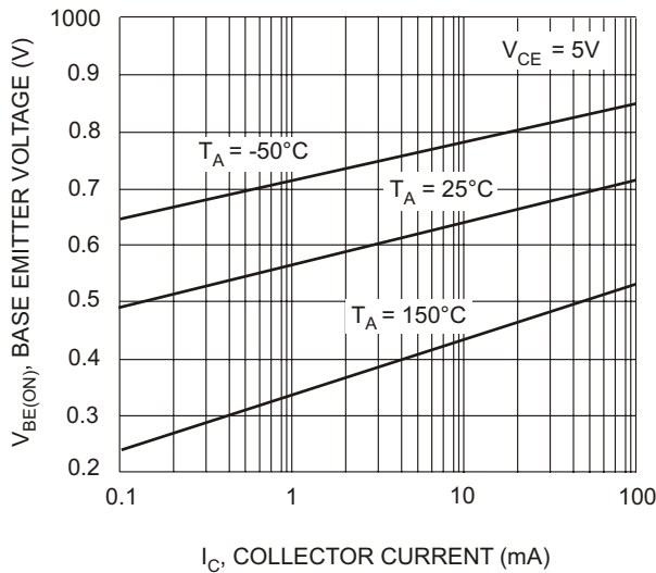
I_C , COLLECTOR CURRENT (mA) Fig. 3 Base-Emitter Voltage vs. Collector Current
