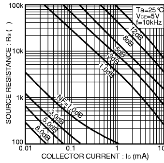
Fig.17 Noise characteristics ( )
