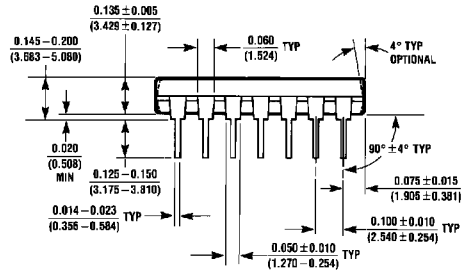
14-Lead Molded Dual-In-Line Package (N) Order Number DM74LS74AN Package Number N14A
