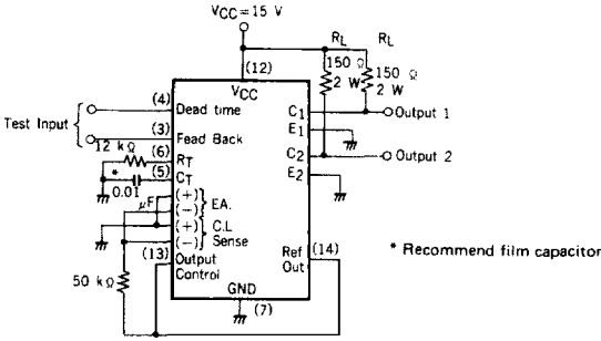
Fig. 1 Test Circuit
