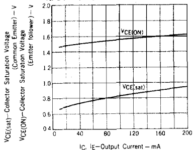
COLLECTOR SATURATION VOLTAGE vs. OUTPUT CURRENT
