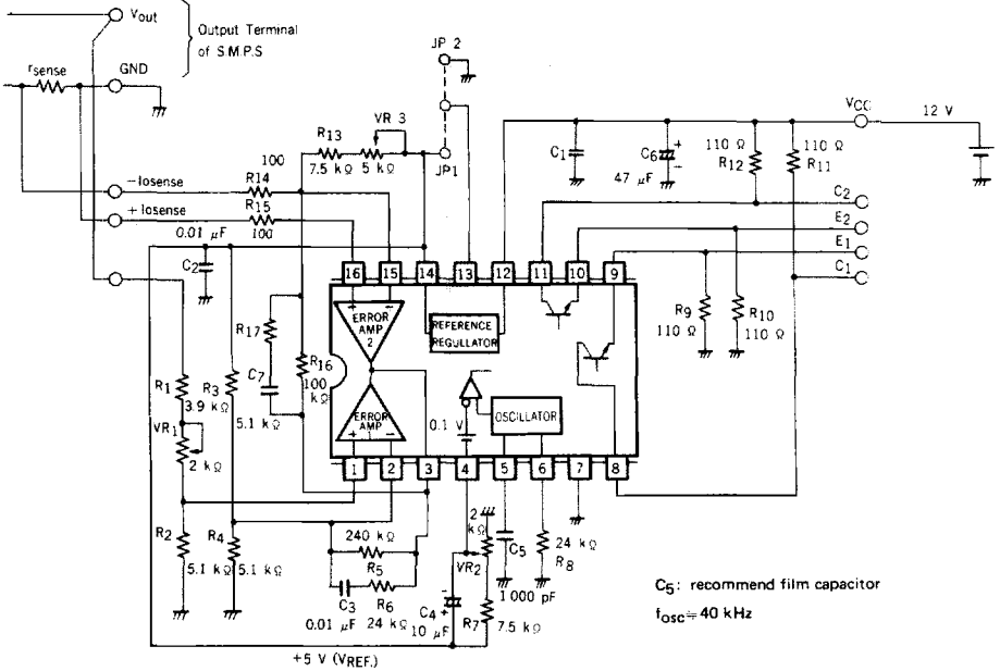
Fig. 2 Circuit
