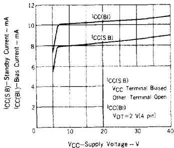
STANDBY AND BIAS CURRENT vs. SUPPLY VOLTAGE
