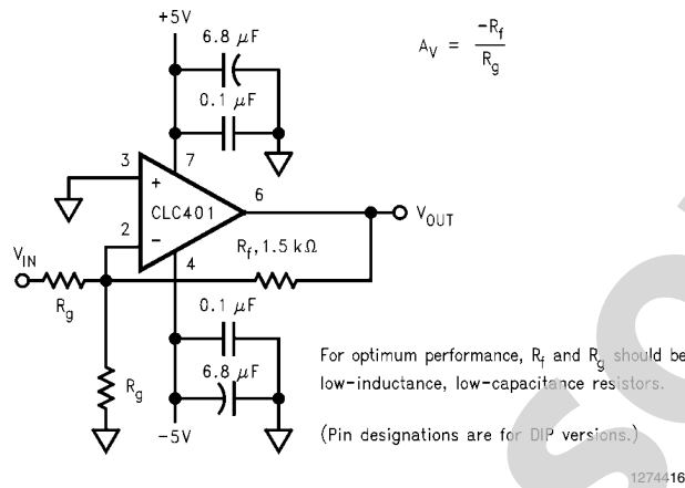
FIGURE 2. Recommended Inverting Gain Circuit
