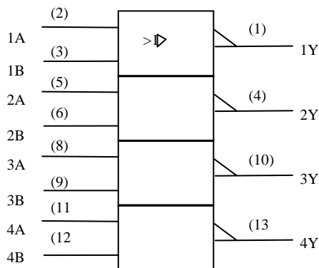
Logic Symbol
