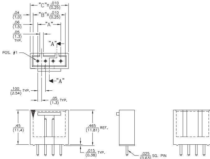
4 THRU 40 POSITION
