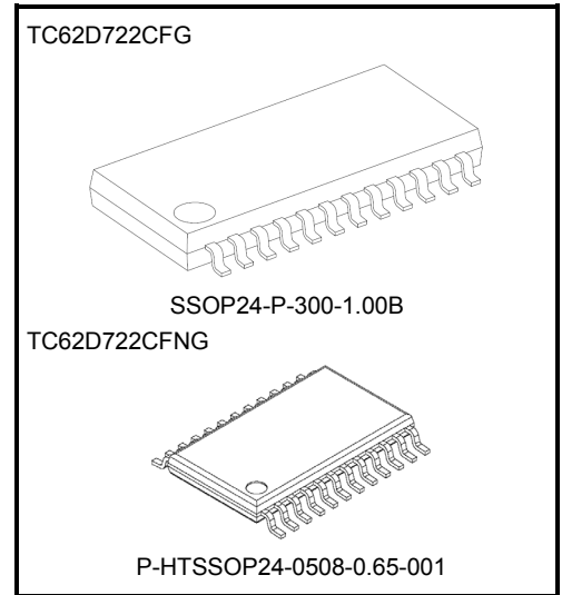
Weight SSOP24-P-300-1.00B : 0.32 g (Typ.) P-HTSSOP24-0508-0.65-001: 0.10 g (Typ.)
