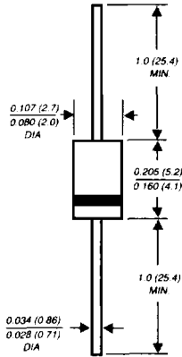
DO-204AL
