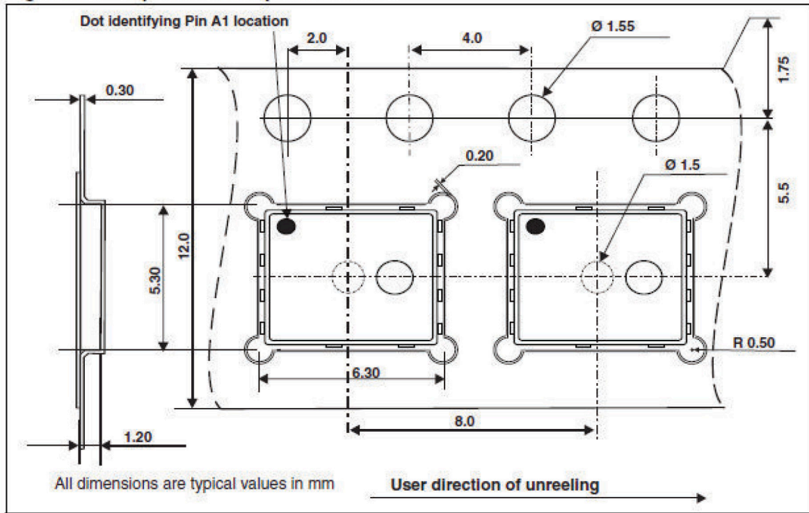
Figure 12. Tape and reel specifications
