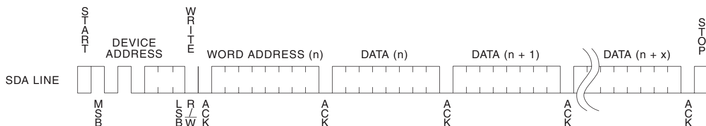
Figure 9. Page Write
