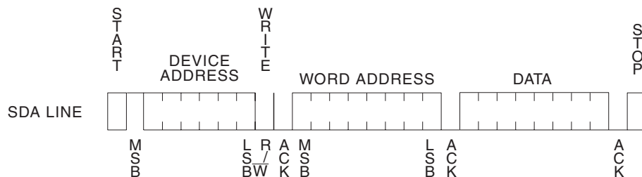
Figure 8. Byte Write
