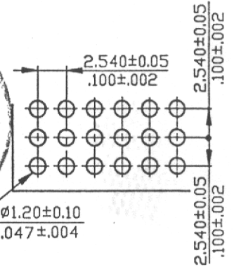
RECOMMENDED HOLE PATTERN
