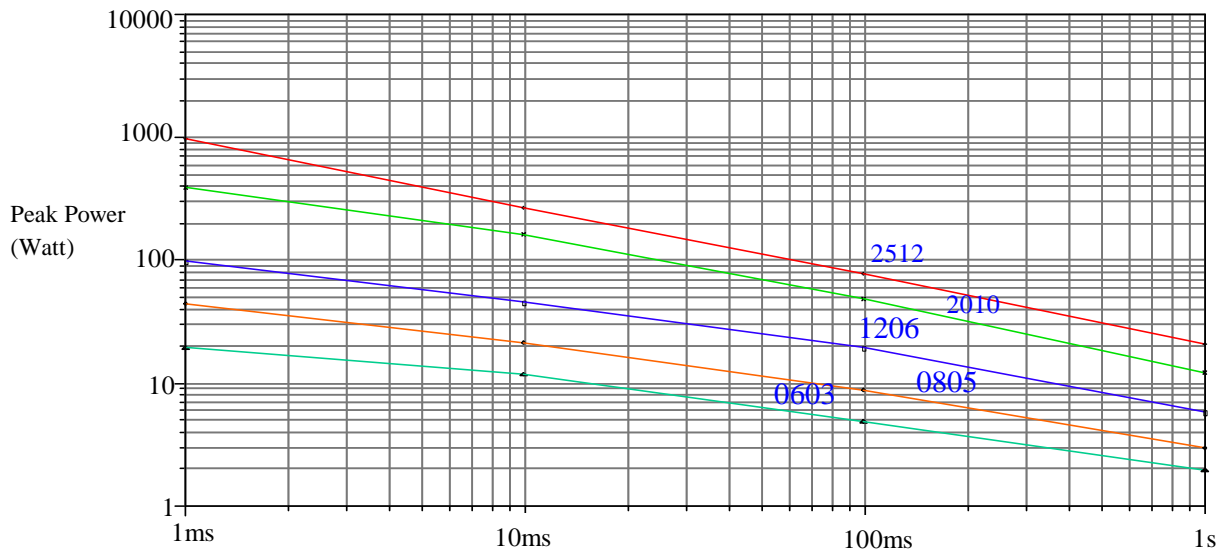
Surge Performance 0603,0805,1206,2010,2512
