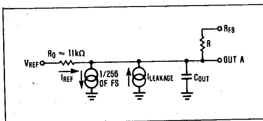
Figure 2. DAC Equivalent Circuit. All Digital Inputs High
