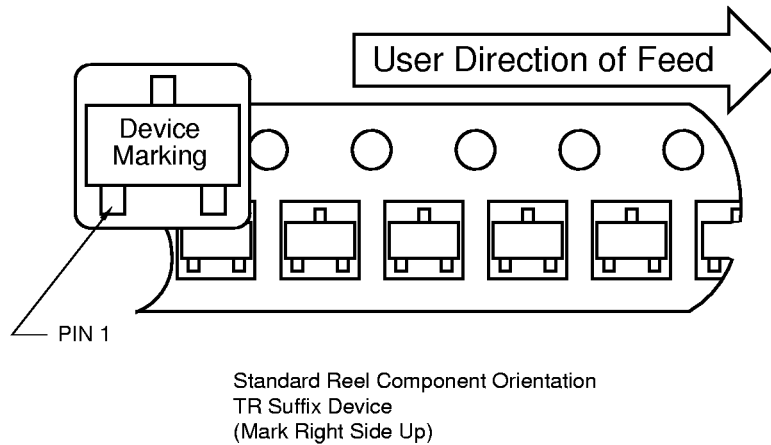
Tape & Reel Specifications Table
