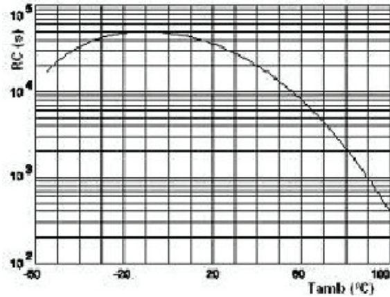
Insulation resistance as a function of the ambient temperature (typical curve)
