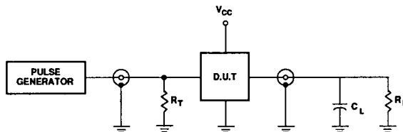
Test Circuit
