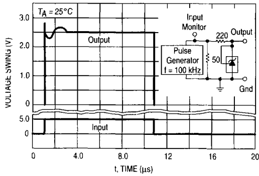
Figure 14. Pulse Response
