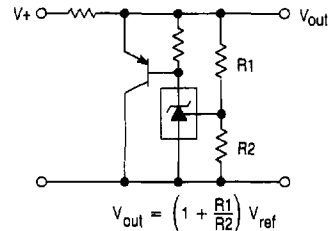
Figure 19. High Current Shunt Regulator
