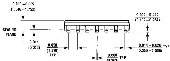
14-Lead Small Outline Molded Package (M) Order Number DM74LS14M Package Number M14A
