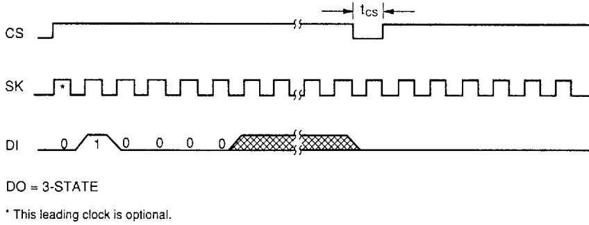
FIGURE 7. WRITE DISABLE (WDS) CYCLE TIMING
