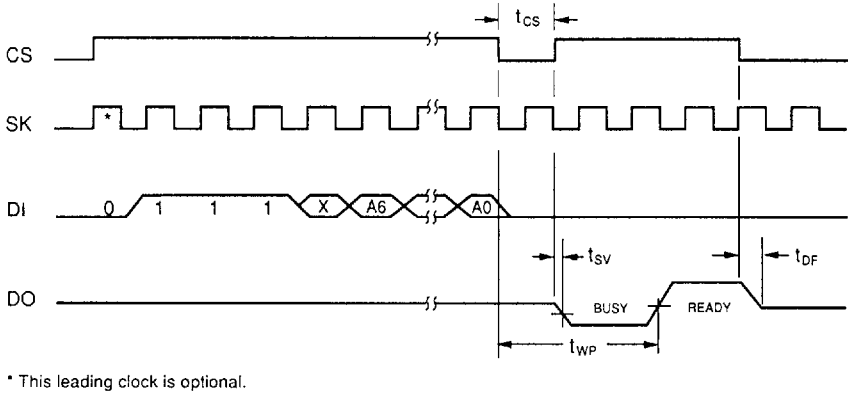
FIGURE 8. ERASE (REGISTER) CYCLE TIMING
