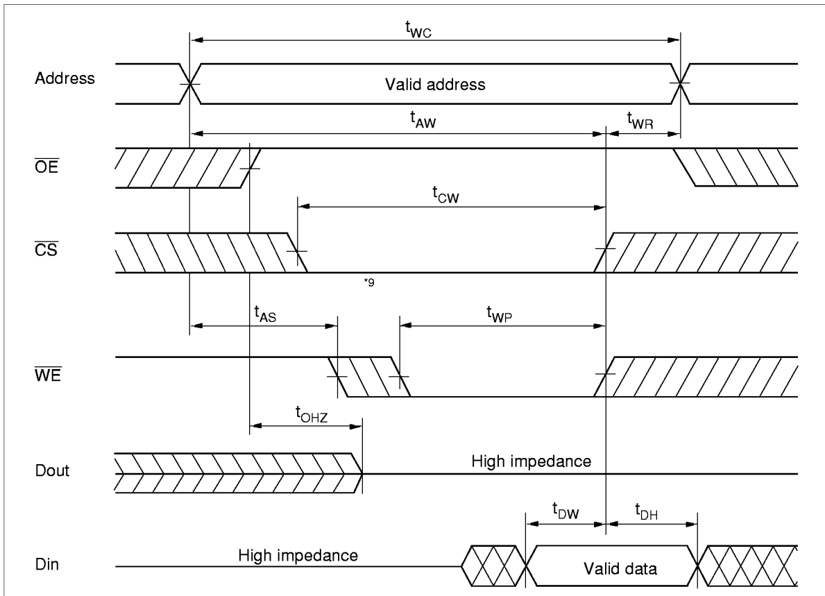
Write Timing Waveform (1) ( \overline{OE} Clock)
