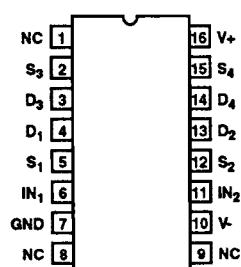
DG303ACY (SOIC) TOP VIEW
