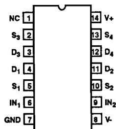
DG302A (CDIP, PDIP) TOP VIEW
