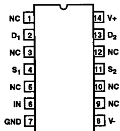
DG301A (CDIP, PDIP) TOP VIEW
