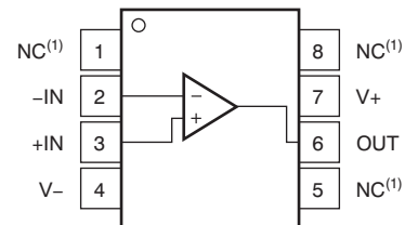
TLV9061 D Package 8-Pin SOIC Top View
