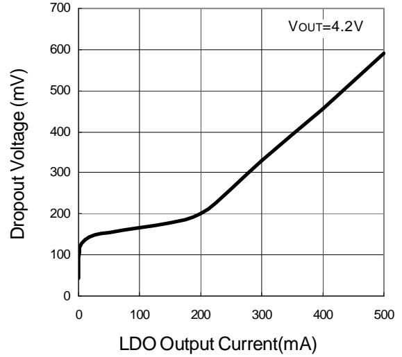
Dropout Voltage vs. LDO Output Current
