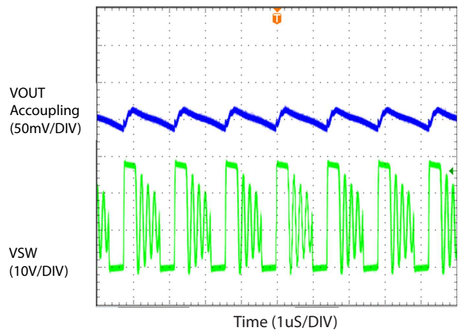
Conditions: VIN = 12V, Output = 27V / 20mA x 4 LED strings
