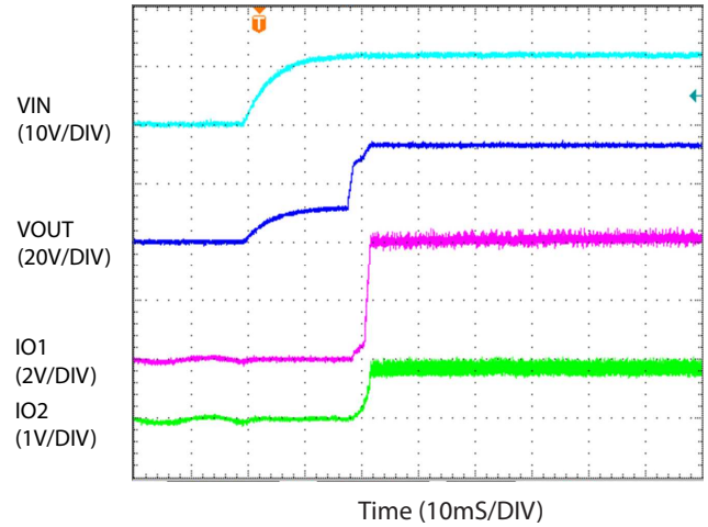
LED Short Circuit Protection
