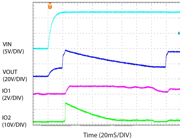
LED Open circuit Protection
