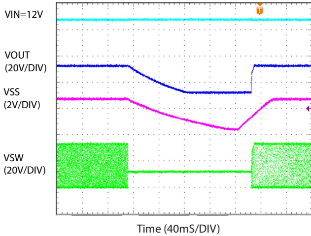
OTP and OTP Recovery
