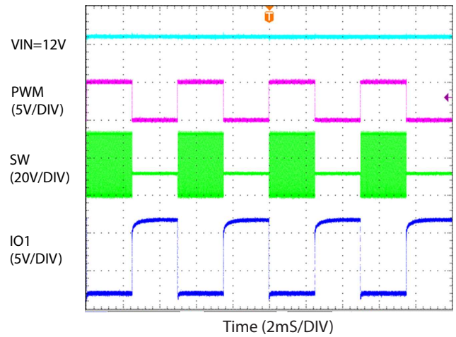
PWM Dimming
