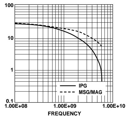
Figure 13. HBFP-0450 Power Gain at 2 V, 10 mA.
