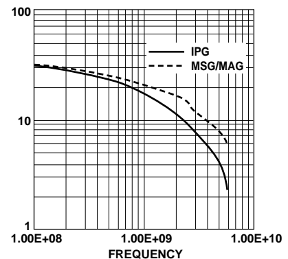
Figure 16. HBFP-0450 Power Gain at 3 V, 50 mA.
