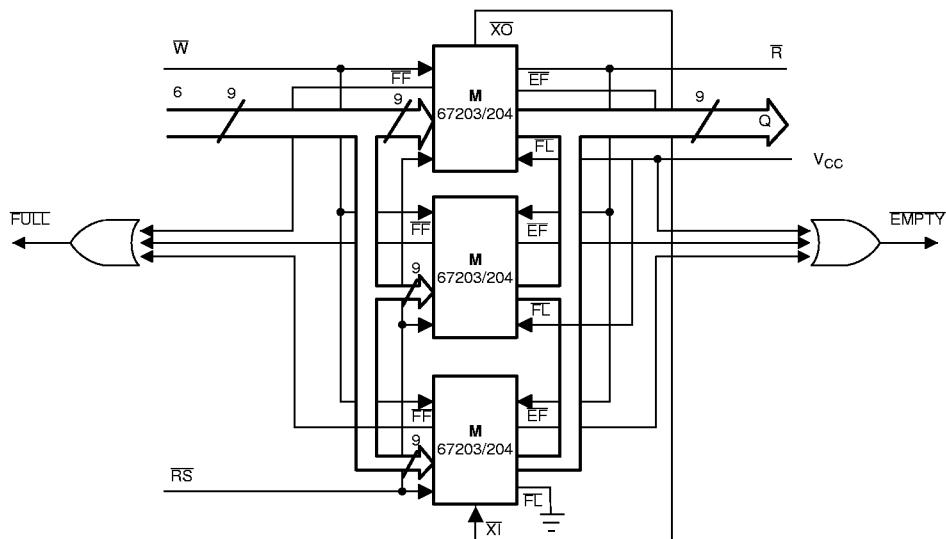
Figure 4. Block Diagram of 6144 \times 9 / 12288 \times 9 FIFO Memory (Depth expansion).
