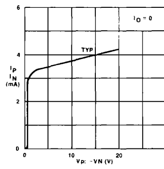
SUPPLY CURRENT
