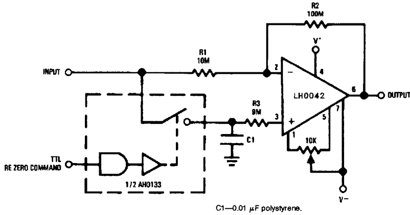
Re-Zeroing Amplifier
