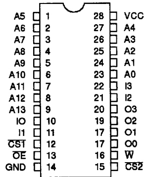
Pinout DIL 28 pins (top view)
