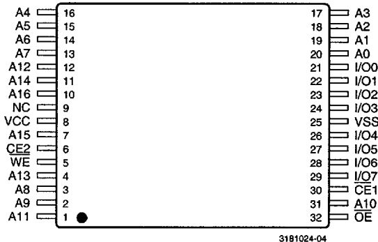
32-Pin TSOP (Reverse)
