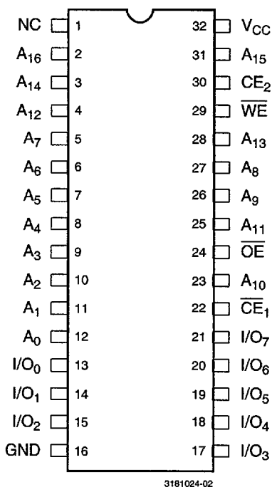
32-Pin DIP/SOP
