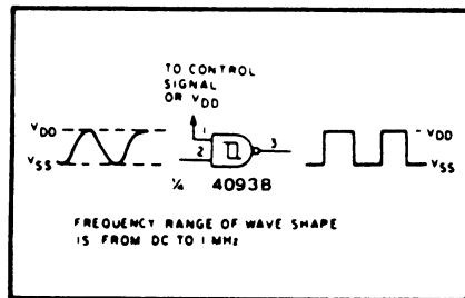
Wave shaper.
