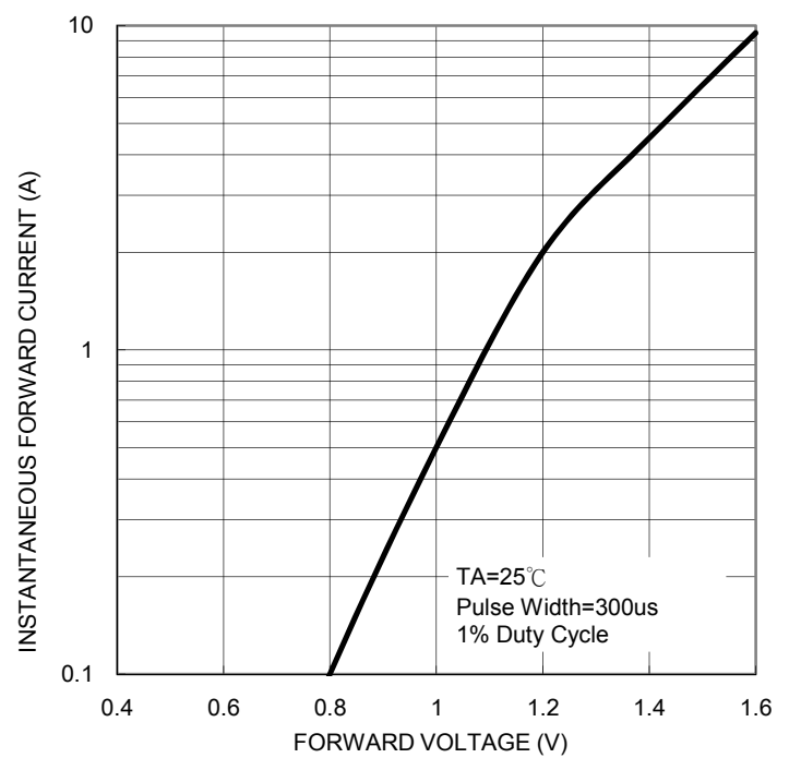
FIG. 5- TYPICAL FORWARD CHARACTERISTICS
