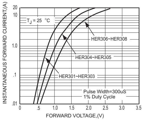
FIG.1-TYPICAL FORWARD CHARACTERISTICS
