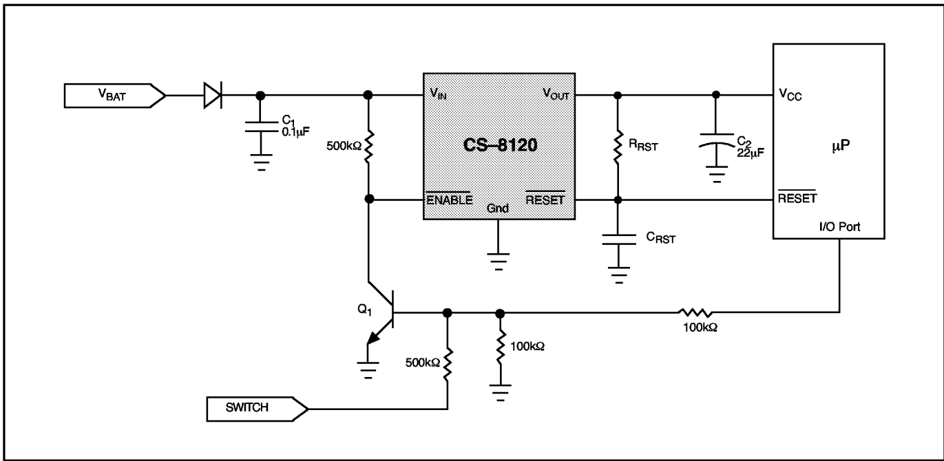
Figure 5: Microprocessor Control of CS-8120 using an external switching transistor (Q1).
