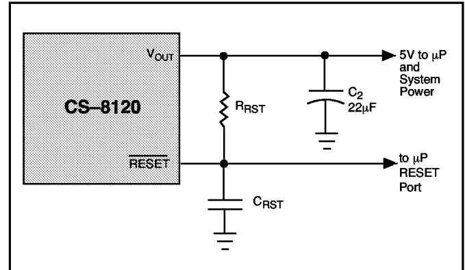
Figure 4: RC Network for RESET Delay circuitry
