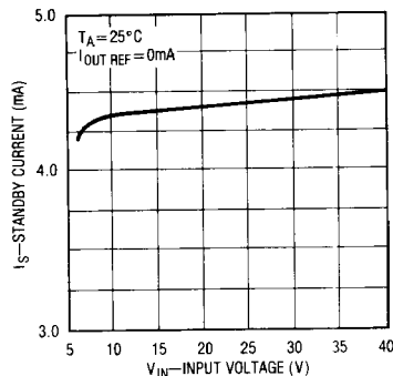
Standby Current
