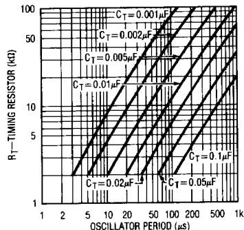
Oscillator Period
