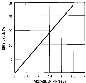
Duty Cycle
