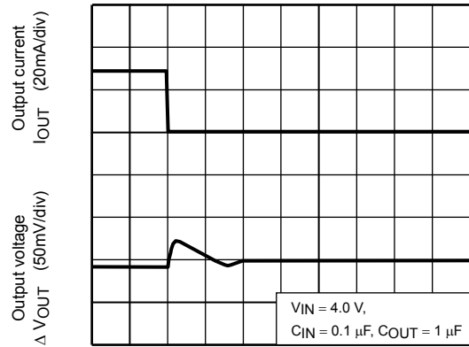
TCR5SB30A ( I_{OUT} = 30\text{m to }1\text{mA} )
