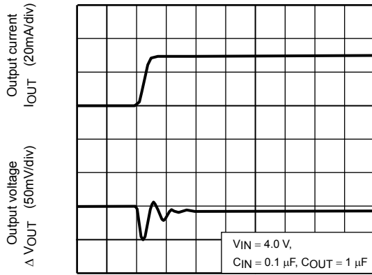
TCR5SB30A ( I_{OUT} = 1\text{m to }30\text{mA} )
