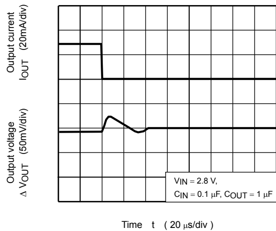
TCR5SB18A (I OUT = 30m to 1mA)
