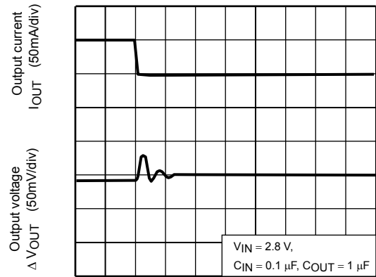
TCR5SB18A ( I_{OUT} = 100\text{m to }50\text{mA} )
