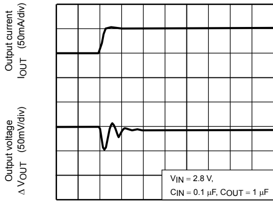
TCR5SB18A ( I_{OUT} = 50\text{m to }100\text{mA} )
