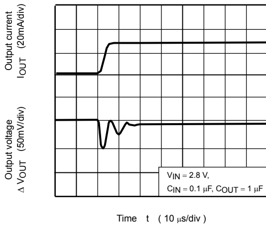
TCR5SB18A (I OUT = 1m to 30mA)
