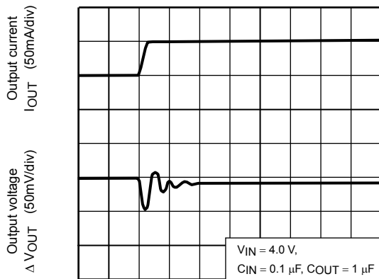
TCR5SB30A ( I_{OUT} = 50\text{m to }100\text{mA} )
