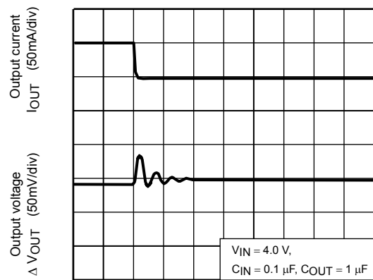
TCR5SB30A ( I_{OUT} = 100\text{m to }50\text{mA} )
