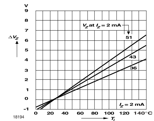
Figure 12. Change of Zener Voltage vs. Junction Temperature
