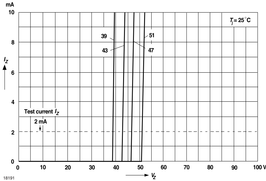
Figure 18. Breakdown Characteristics
