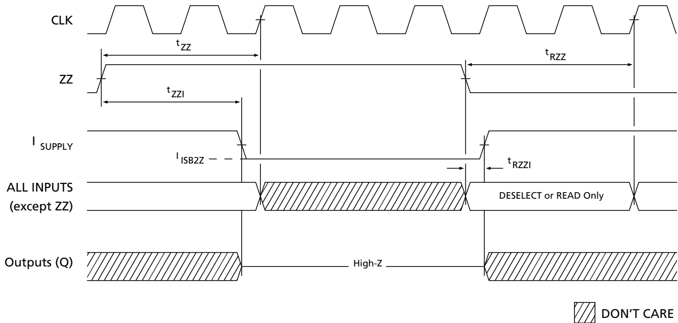
Figure 10: SNOOZE MODE Waveform
