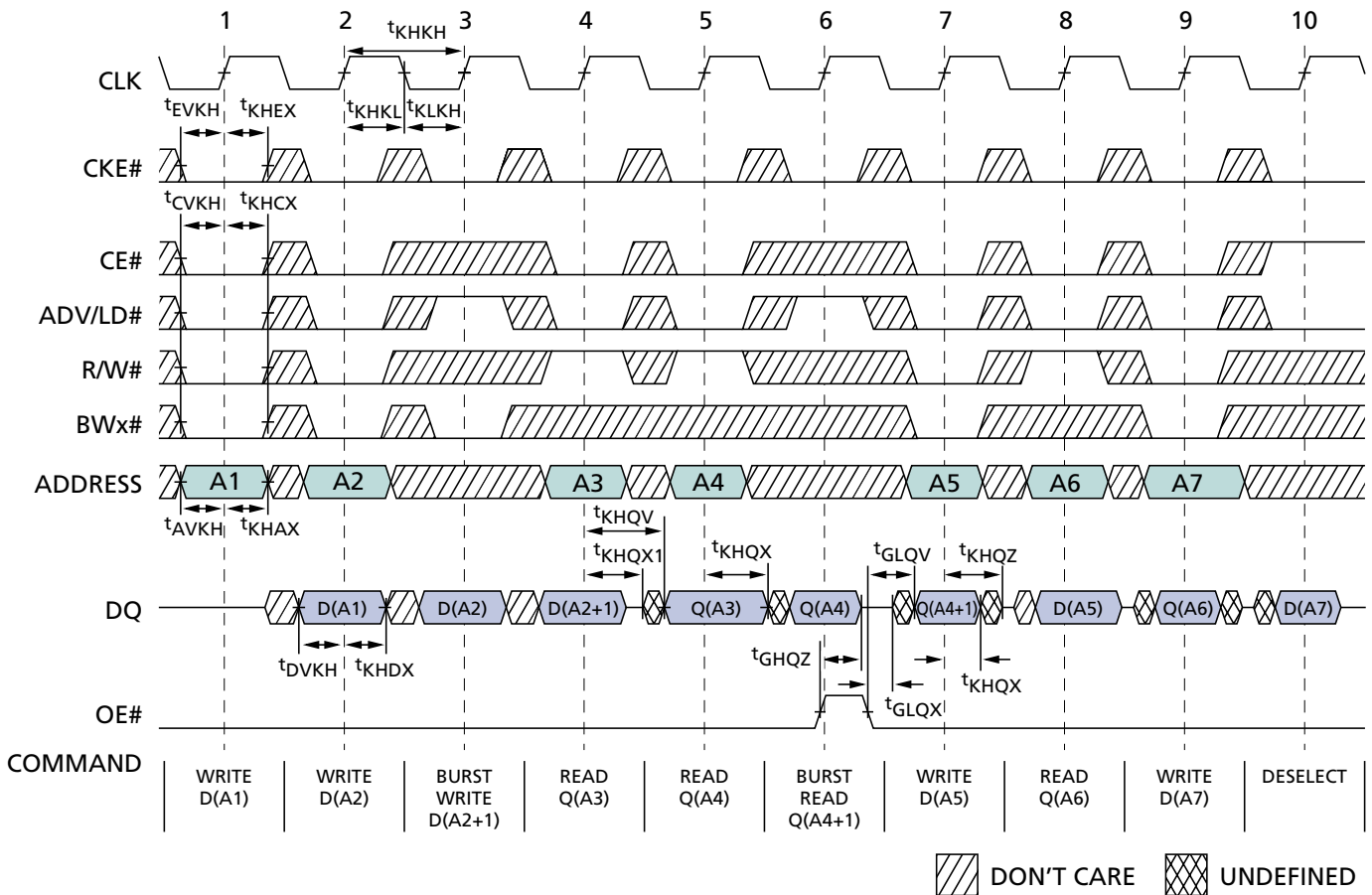
Figure 8: READ/WRITE Timing
