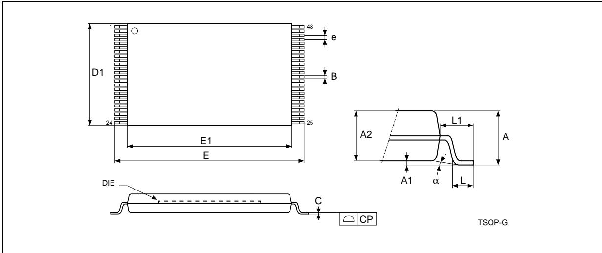
Figure 14. TSOP48 - 48 lead Plastic Thin Small Outline, 12 x 20mm, Package Outline
